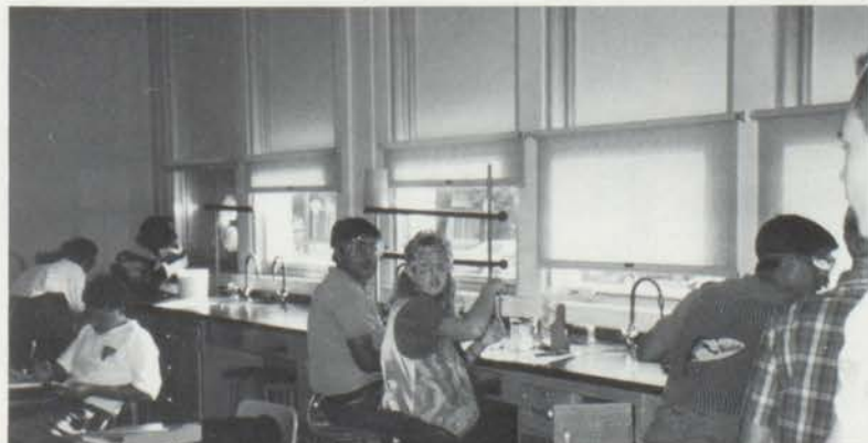
Avogadros number?
