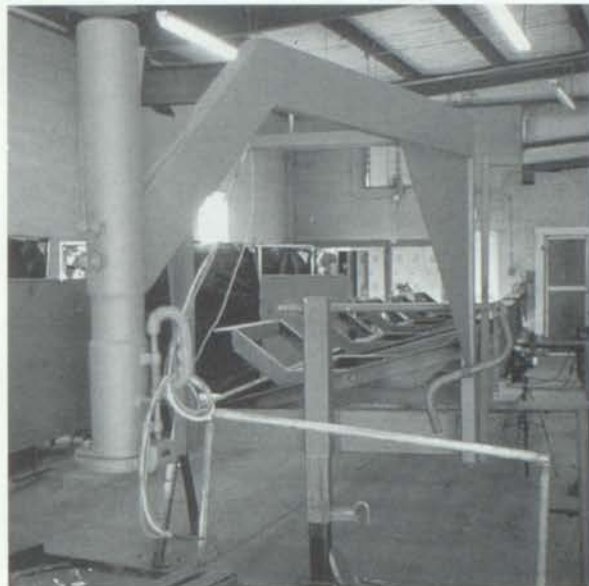
5-Bale Gooseneck Haytrailer built by Ag Mechanics class.
